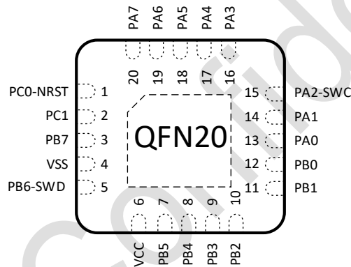
Figure 3-2 QFN20 Pinout1 PY32L020F15U
