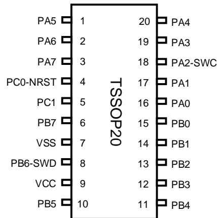
Figure 3-1 TSSOP20 Pinout1 PY32L020F15P
