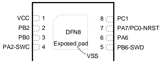
Figure 3-3 DFN8 Pinout1 PY32L020L15D
