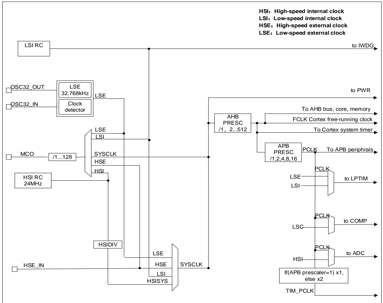
Figure 2-1 System Clock Structure Diagram
