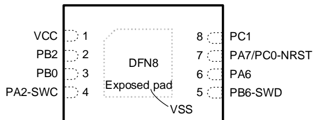
图 3-3 DFN8 Pinout1 PY32L020L15D
